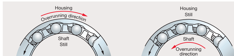
Fig. 2 When Clutch is Overrun
